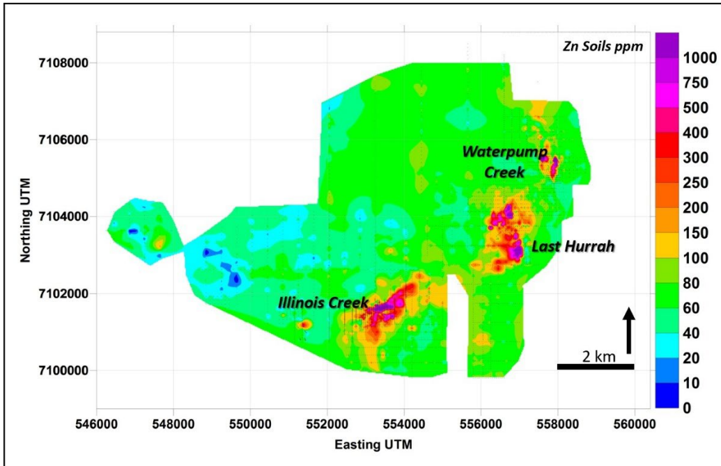
Figure 9.2: Zinc Soil Geochemistry - Illinois Creek Property
