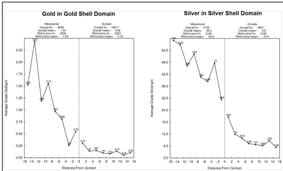
Figure 14.10: Contact Profiles of Gold and Silver Grades Across Grade Shell Domain Boundaries
