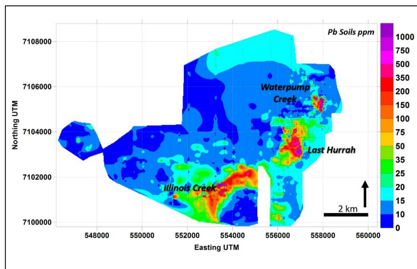
Figure 9.1: Lead Soil Geochemistry - Illinois Creek Property
