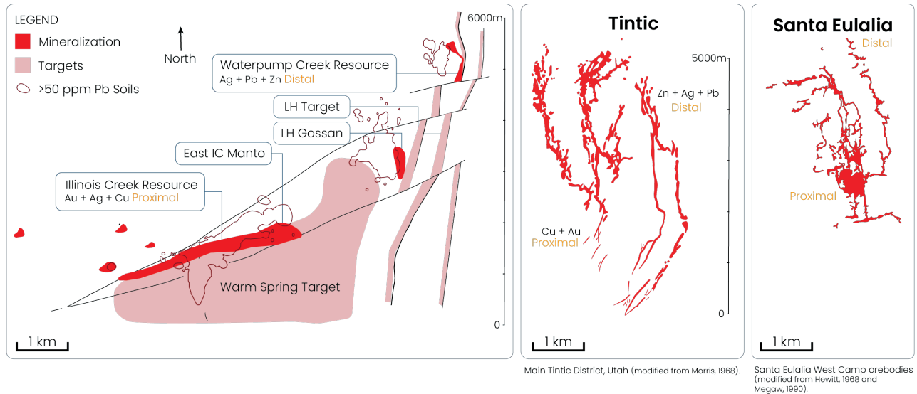
Figure 8.1: Comparison of Illinois Creek CRD System with Major Worldwide CRD Systems
