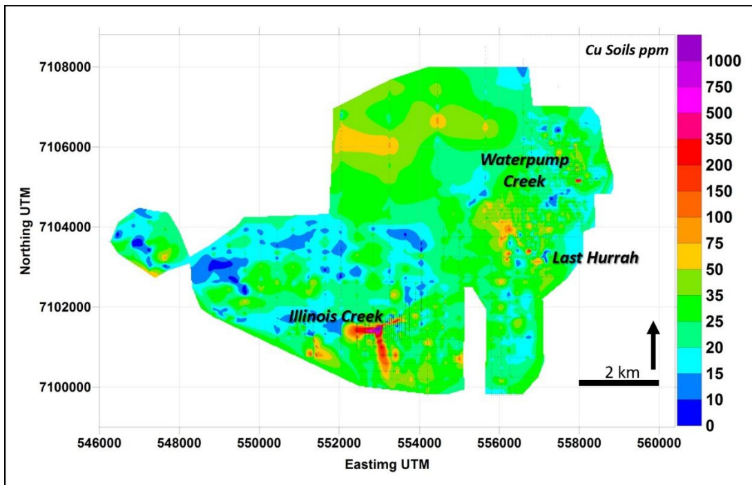
Figure 9.5: Copper Soil Geochemistry - Illinois Creek Property
