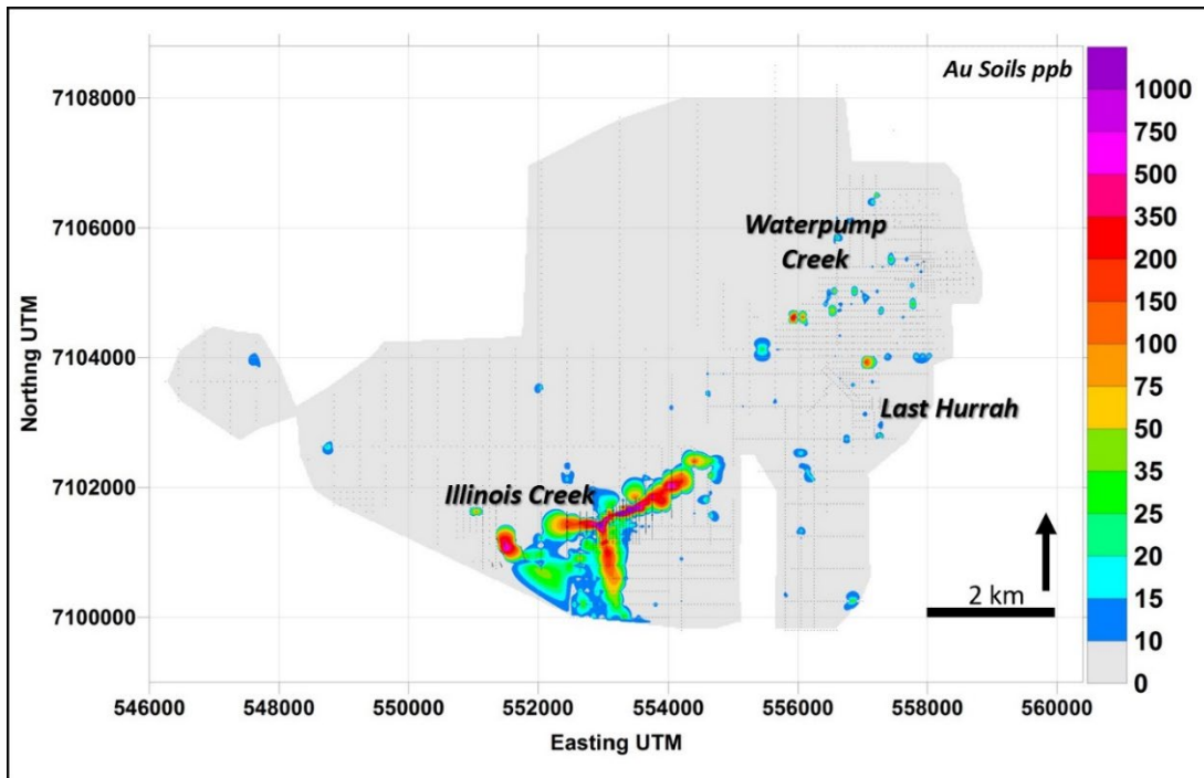
Figure 9.4: Gold Soil Geochemistry - Illinois Creek Property
