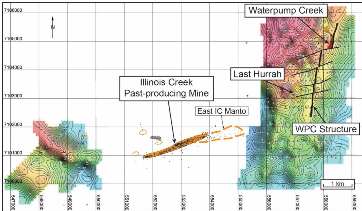
Figure 6.5: 2004 NovaGold/Edcon Gravity Survey
