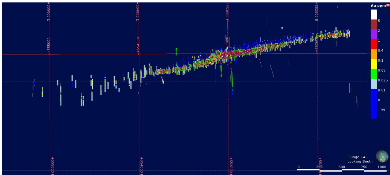
Figure 7.18: 3D perspective view of the Illinois Creek deposit showing gold grades
