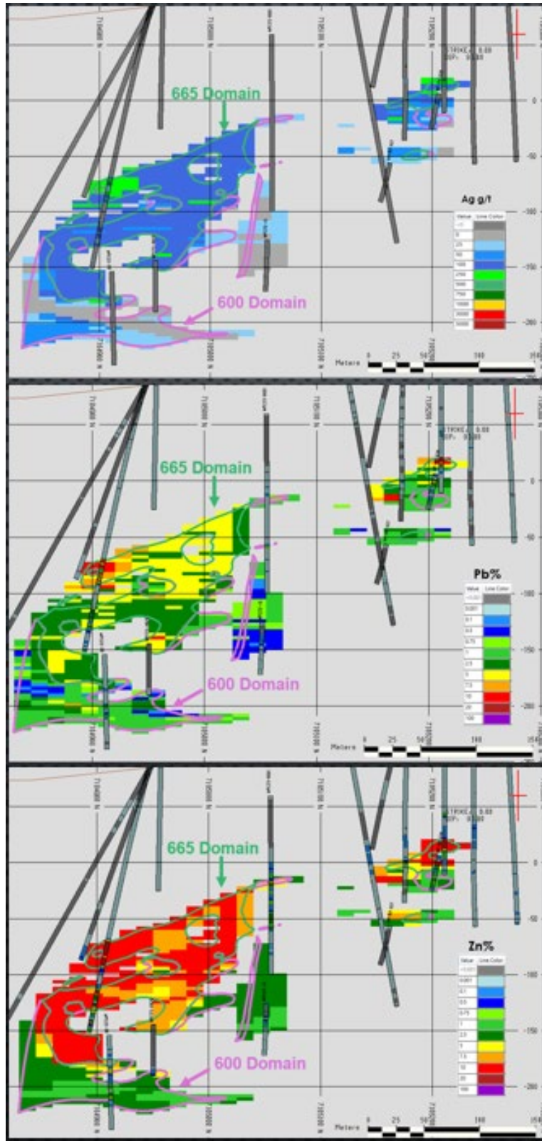
Figure 14.41: Grades in Drilling and Block Model, Section 558255E, Domains 600 and 665
