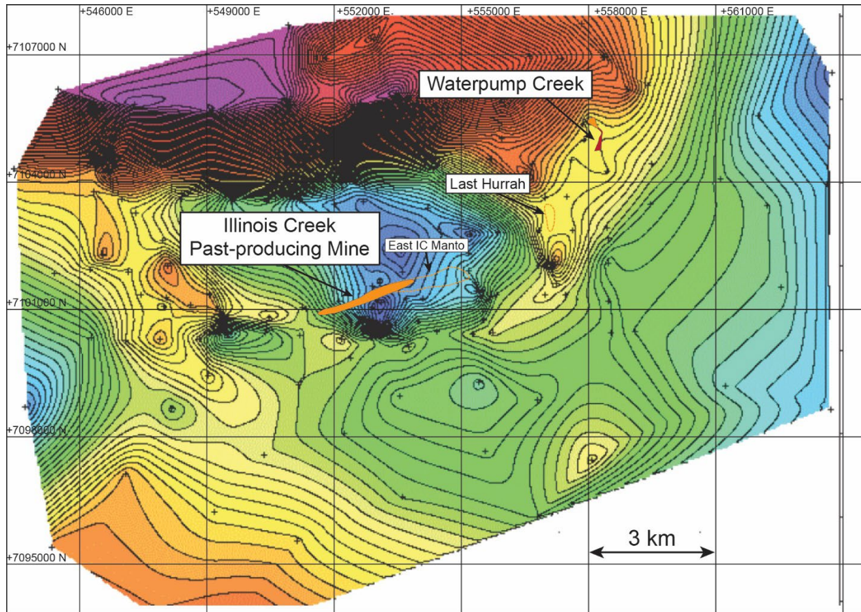
Figure 6.4: Regional Gravity Survey (Edcon, 1983)
