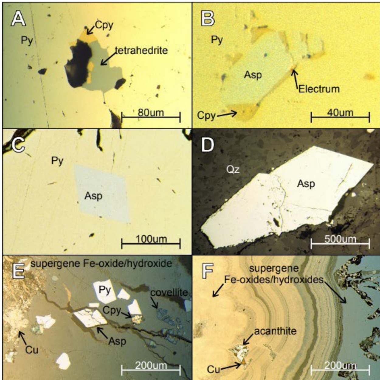
Figure 7.20: Reflected light photomicrographs of rare primary minerals at Illinois Creek
