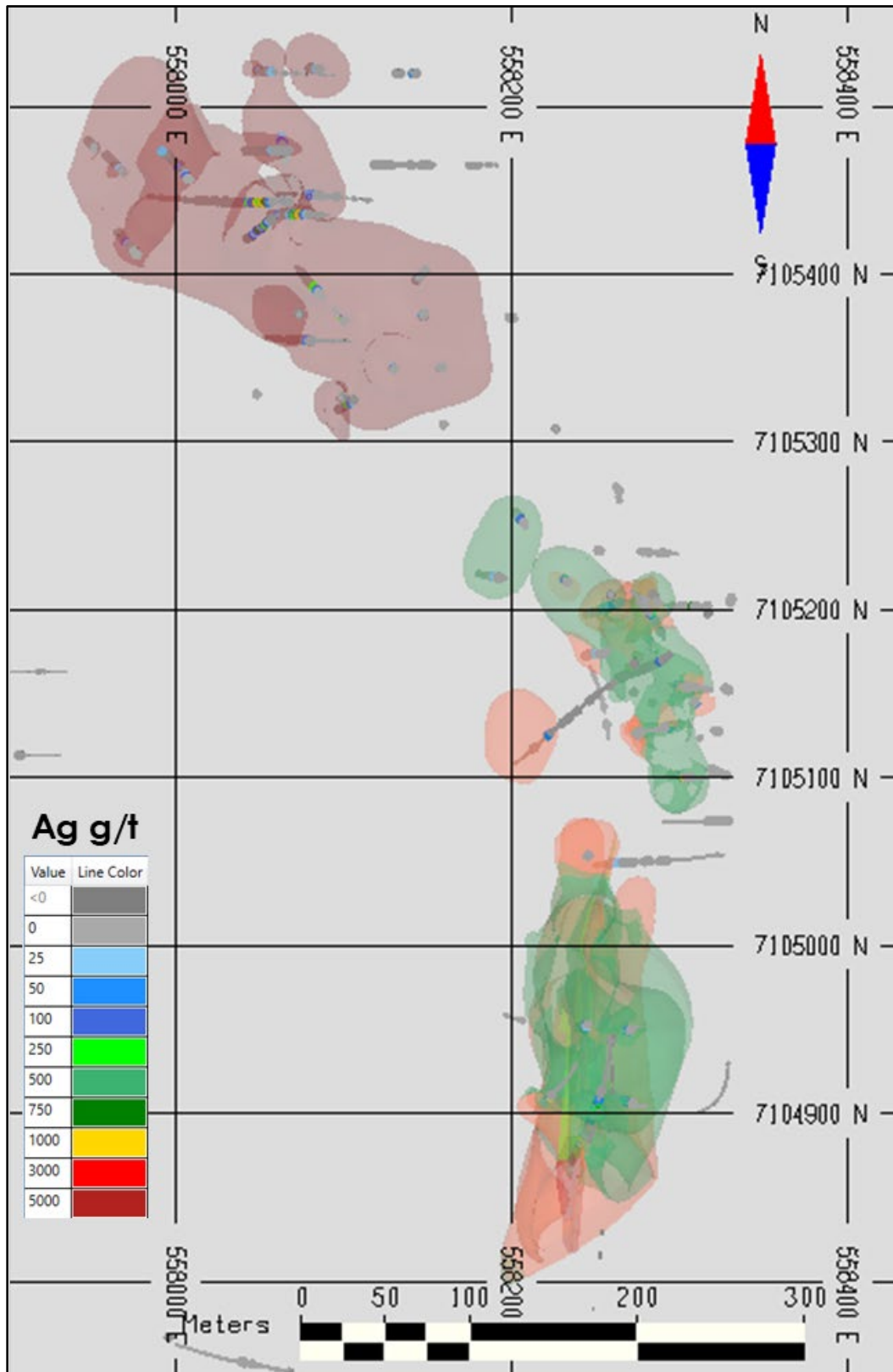
Figure 14.31: Plan View of Silver Grades in Drilling, Ag g/t
