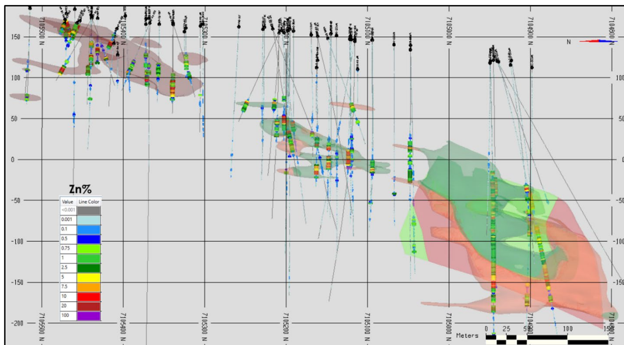
Figure 14.36: Long Section View of Zinc Grades in Drilling, Zn %
