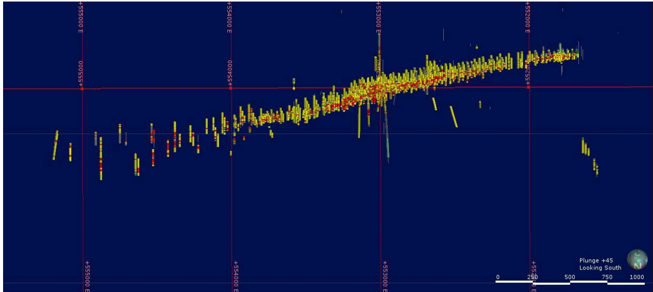
Figure 7.17: 3D Perspective View of Illinois Creek Deposit Showing FG and FQ Units (Red) and Calcareous and Dolomitic Quartzites (Yellow)
