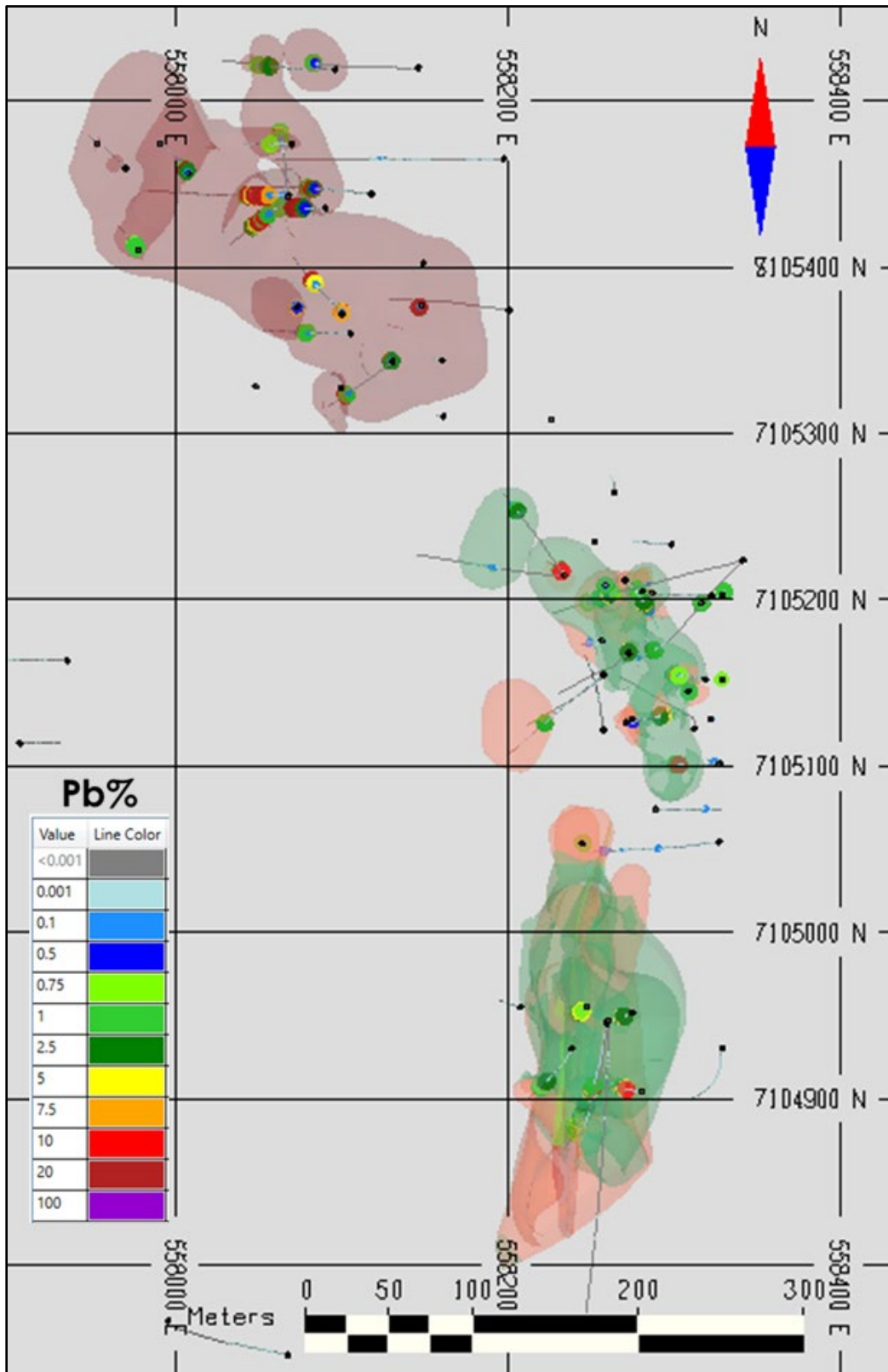
Figure 14.33: Plan View of Lead Grades in Drilling, Pb %
