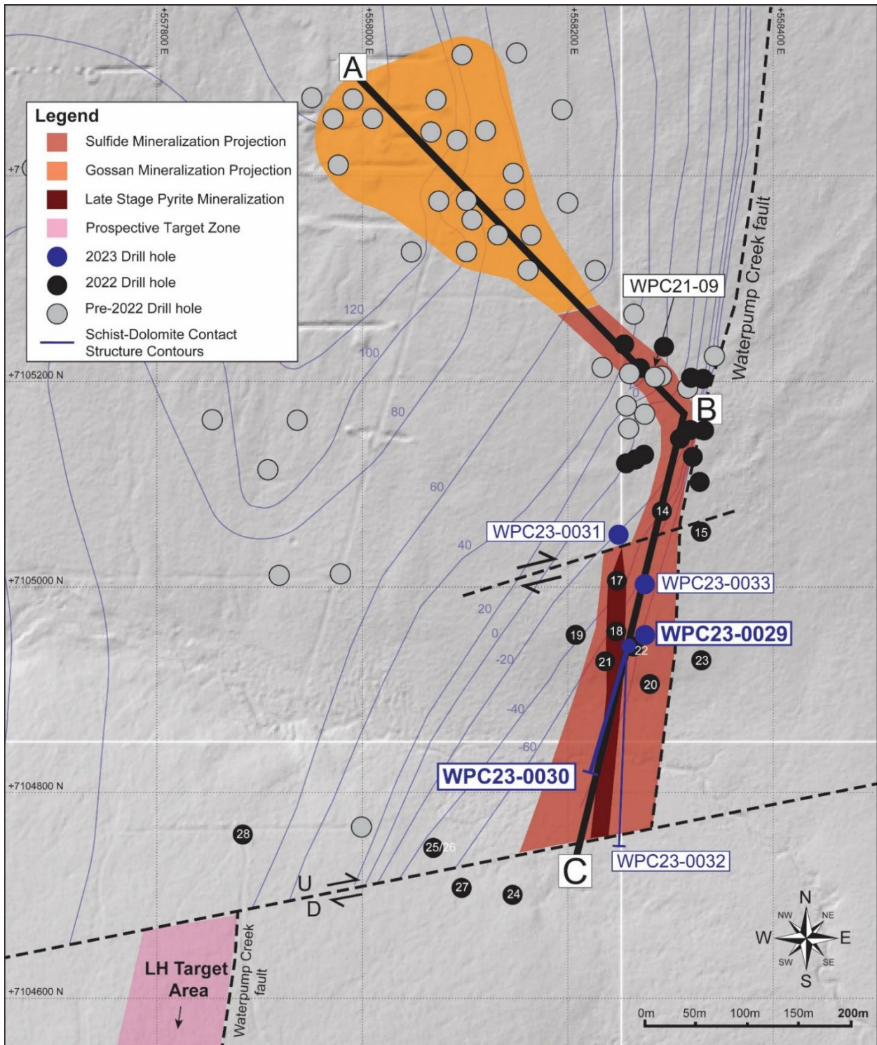
Figure 7.7: Plan Map of the Waterpump Creek Drill Collars
