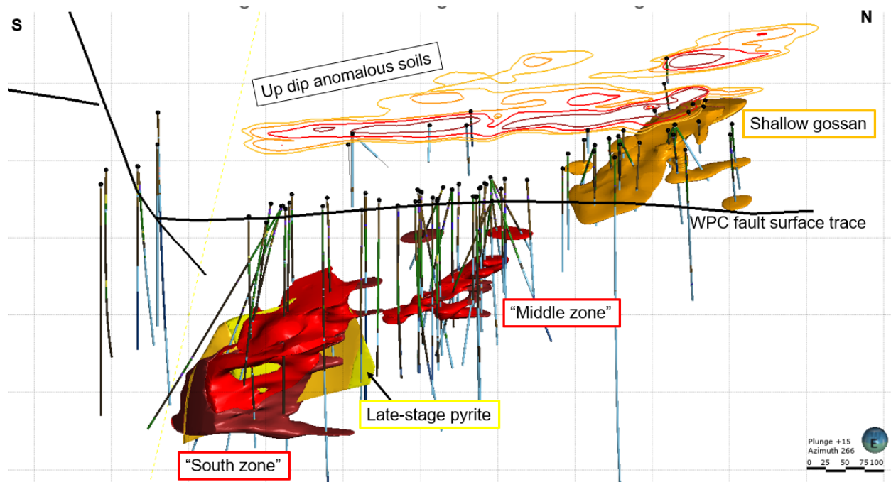
Figure 7.9: 3D Plan Map Projection of the Waterpump Creek Sulfide Body
