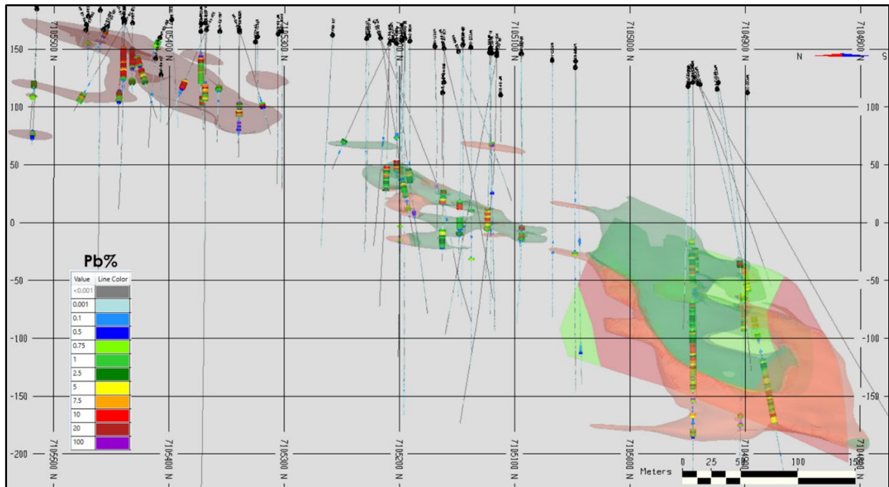
Figure 14.34: Longsection View of Lead Grades in Drilling, Pb %
