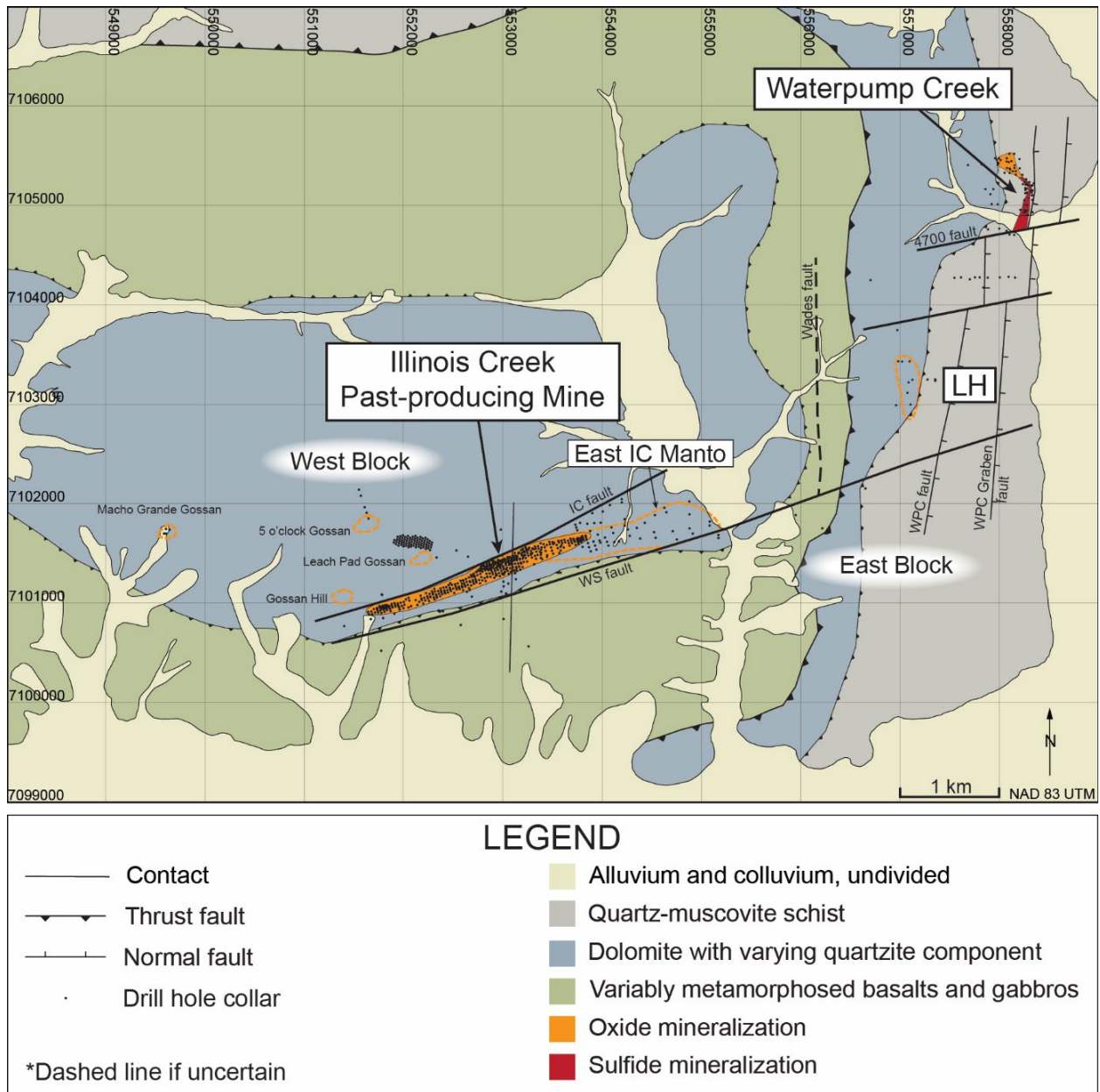
Figure 7.6: Simplified Geologic Map of the Illinois Creek Property with Primary Mineralization-controlling Structures and Simplified Geologic Domains
