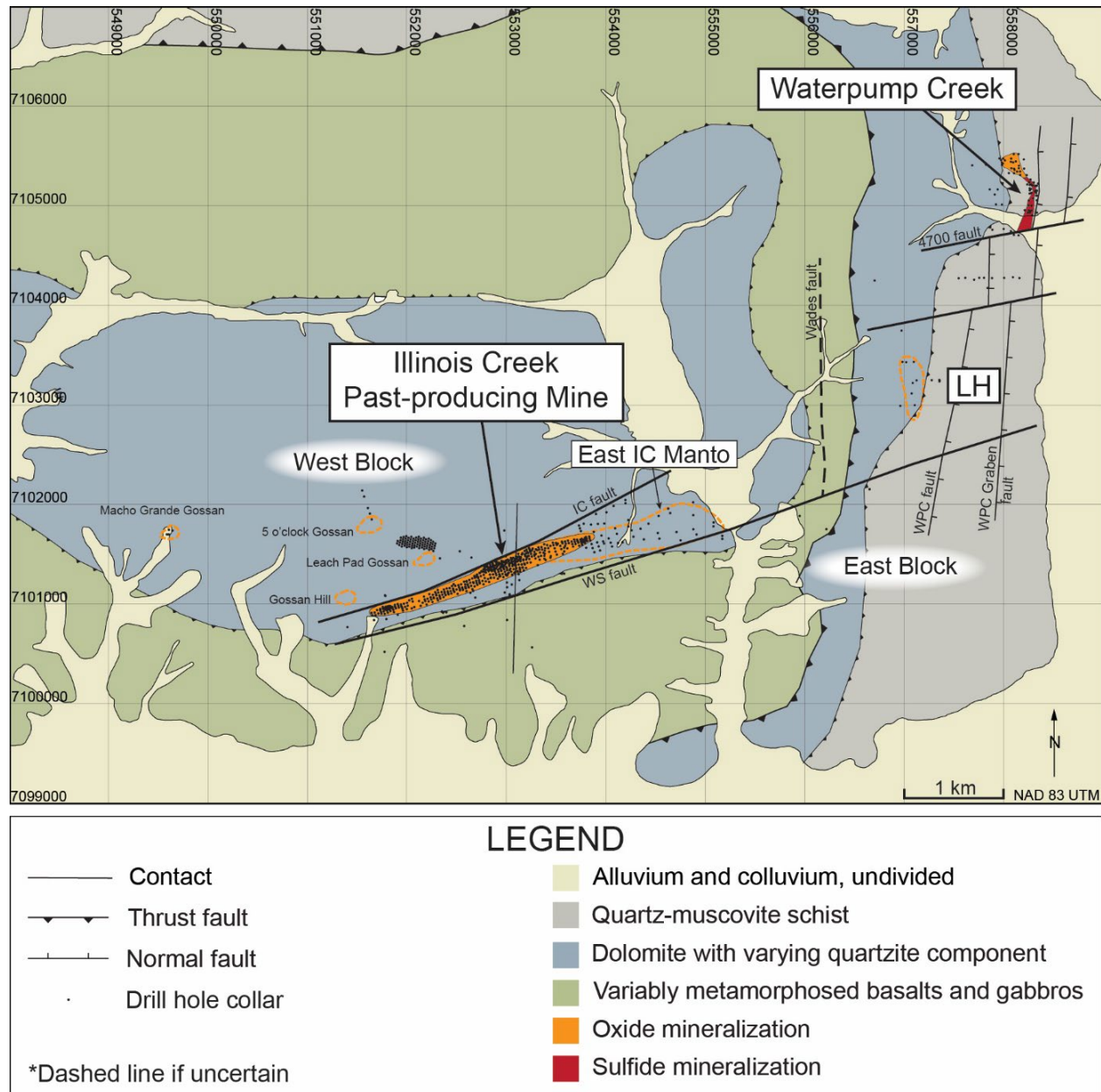
Figure 6.1: Simplified plan map showing mineralized zones, drill collars, simplified map units, and major mineralization-controlling structures
