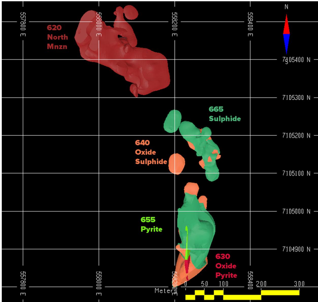
Figure 14.37: Plan View of Mineralized Domains at Waterpump Creek Deposit
