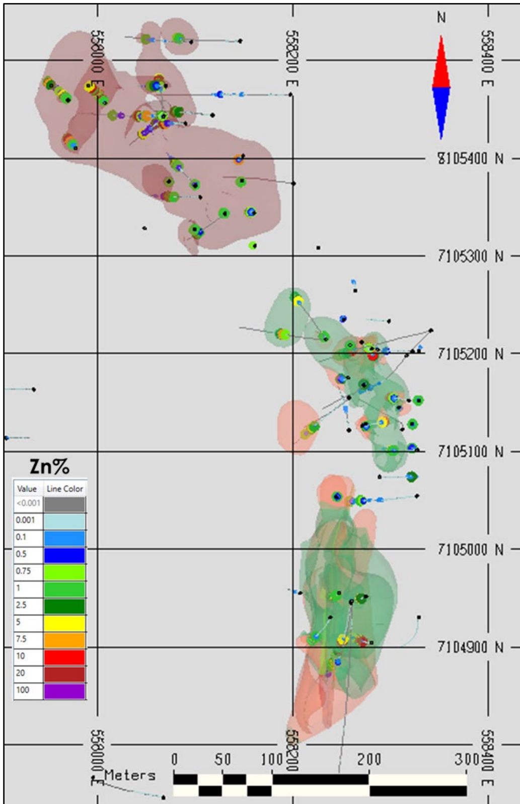
Figure 14.35: Plan View of Zinc Grades in Drilling, Zn %
