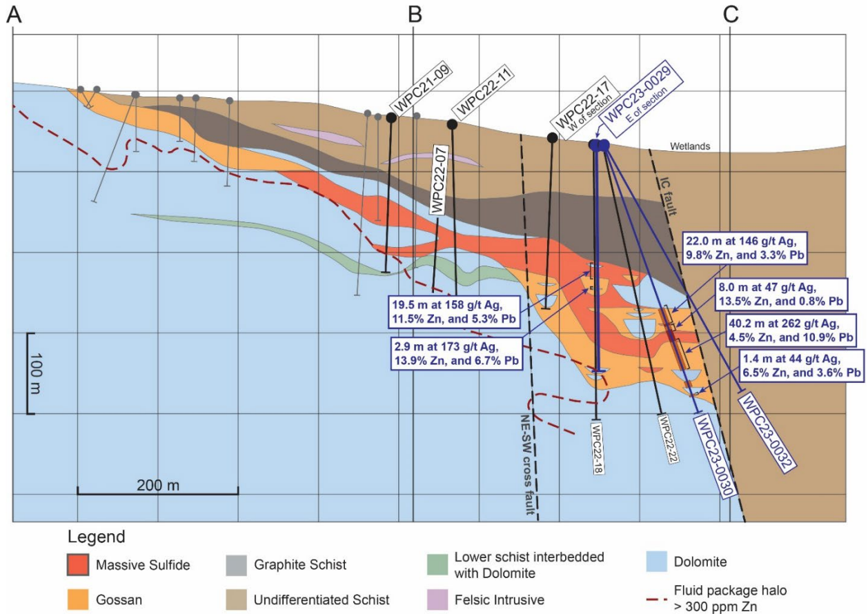
Figure 7.8: Longitudinal Section Down Axis of Waterpump Creek Manto
