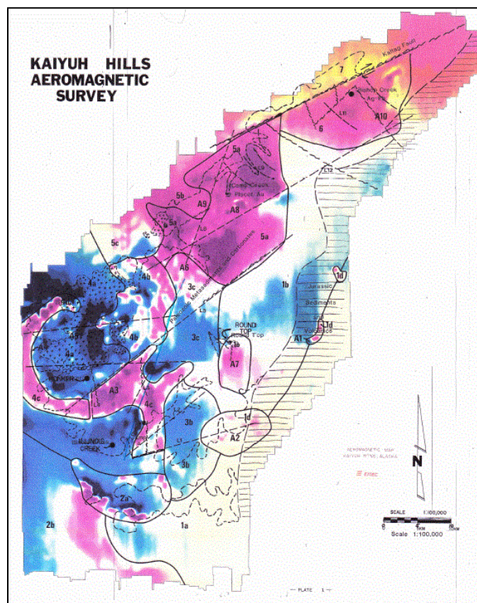
Figure 6.2: Total Field Magnetics - Kaiyuh Hills (Ertec, 1982)
