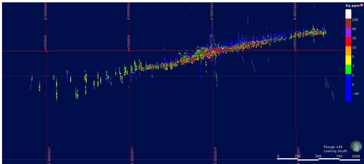
Figure 7.19: 3D perspective view of Illinois Creek Deposit showing silver grades
