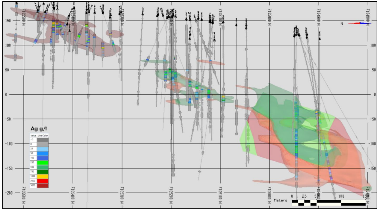
Figure 14.32: Long Section View of Silver Grades in Drilling, Ag g/t
