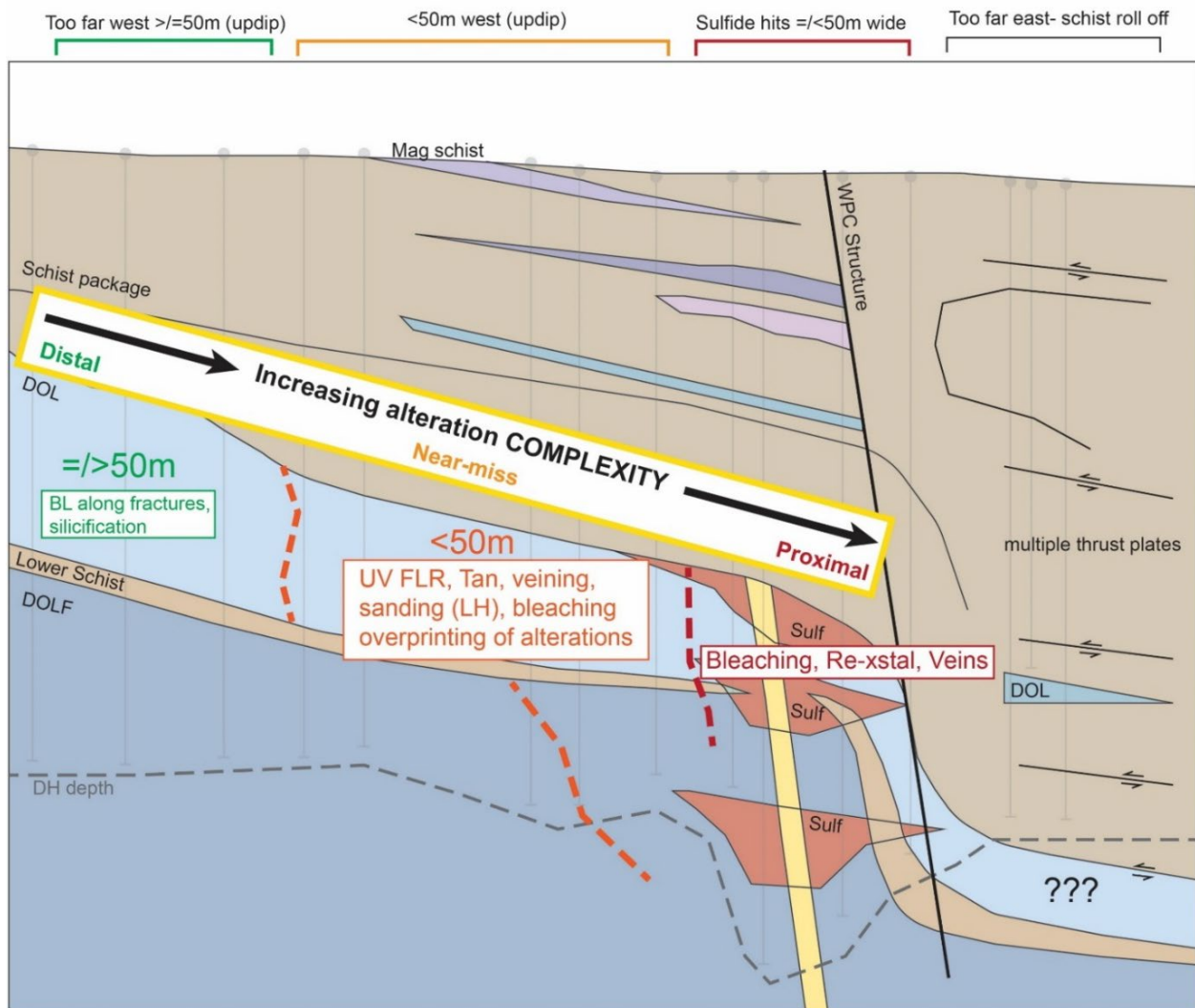
Figure 7.22: Schematic Cross-Section Showing the Alteration Zonation of WPC
