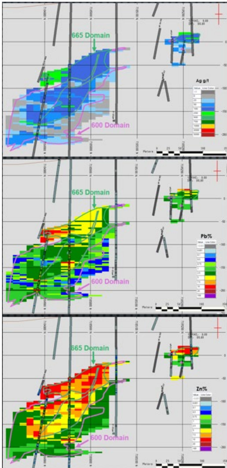
Figure 14.40: Grades in Drilling and Block Model, Section 558240E, Domains 600 and 665
