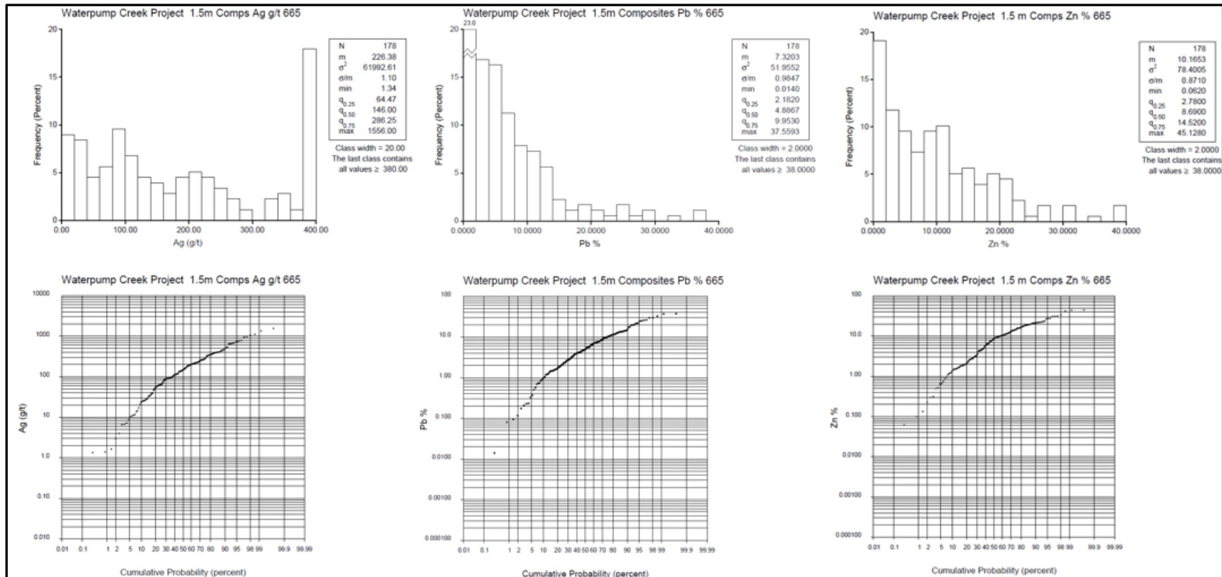
Figure 14.39: Histogram/Probability Plots of 1.5 m Composites for Ag g/t, Pb% and Zn% in Domain 665
