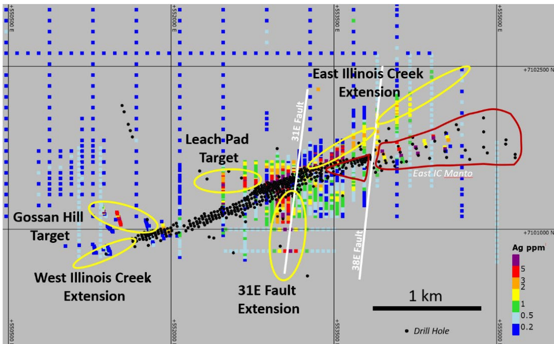
Figure 9.7: Silver Soil Geochemistry and Oxide Exploration Targets Near the Illinois Creek Deposit
