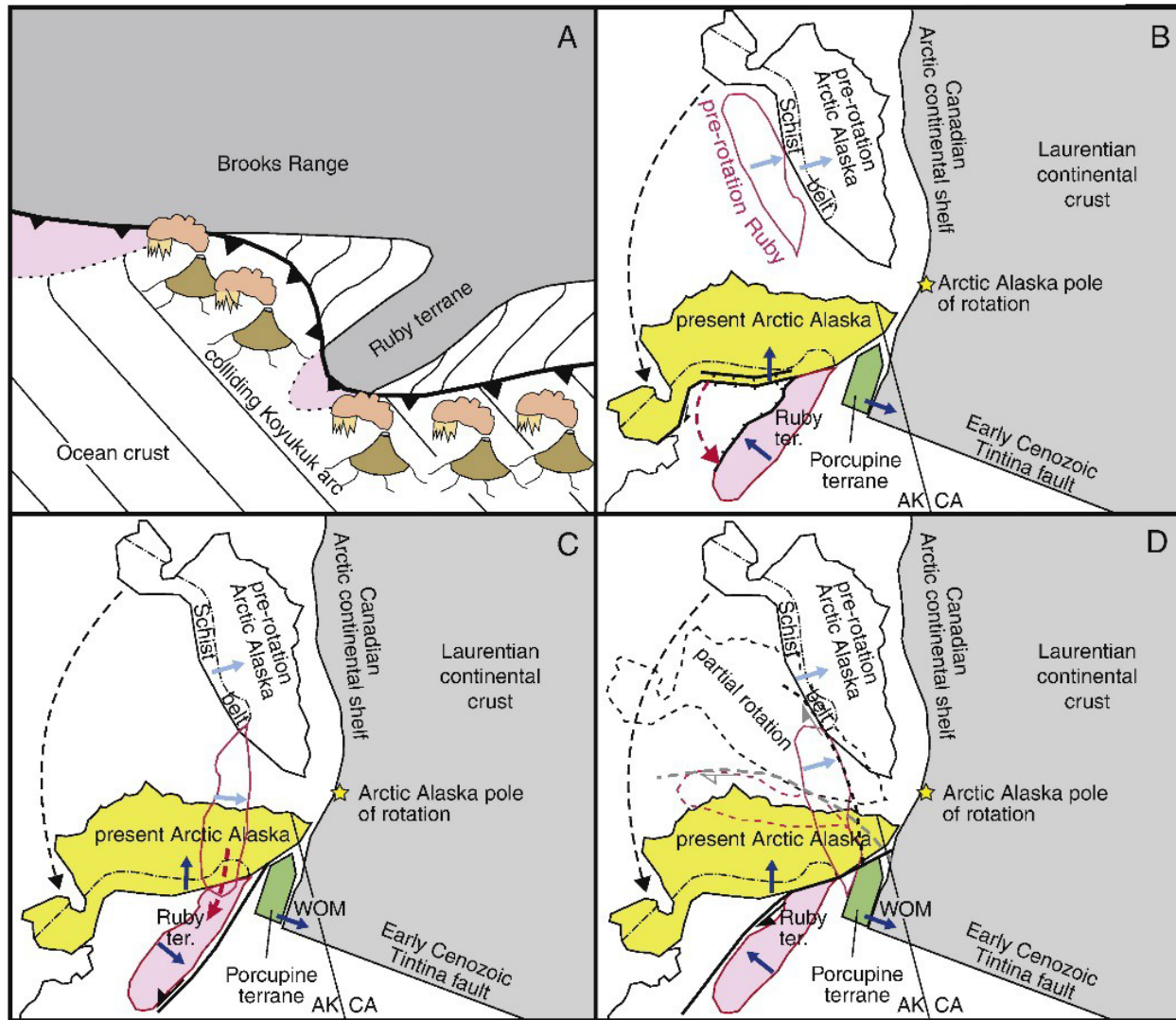
Figure 7.2: Existing Tectonic Models for the Ruby Terrane
