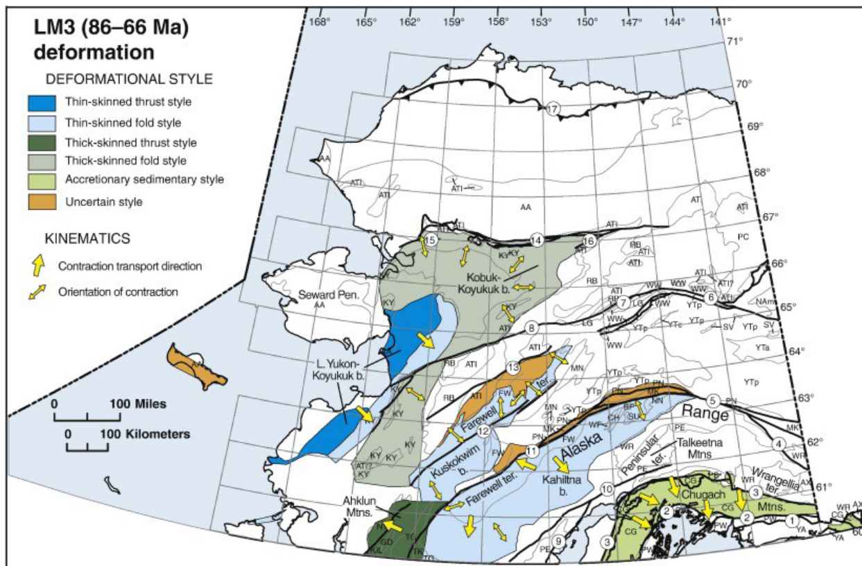
Figure 7.5: West-Central Alaska Deformation 86-66 Ma
