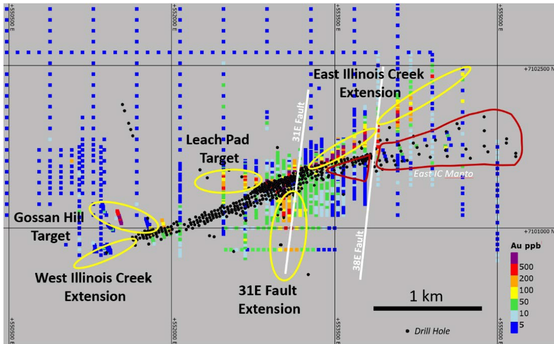
Figure 9.6: Gold Soil Geochemistry and Oxide Exploration Targets Near the Illinois Creek Deposit
